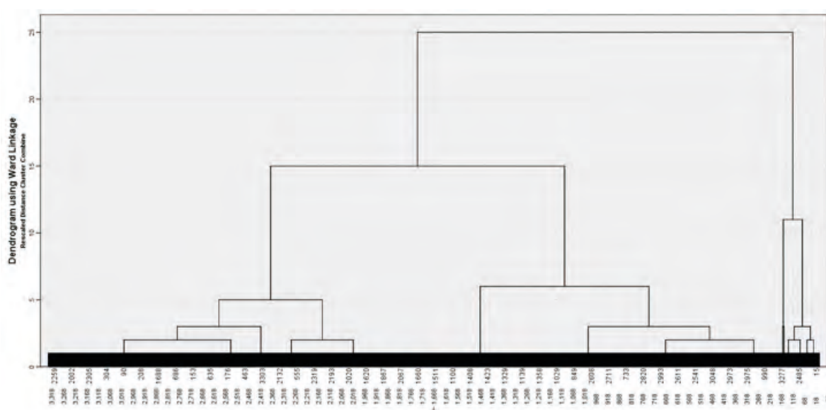
Graph 1. Dendrogram
