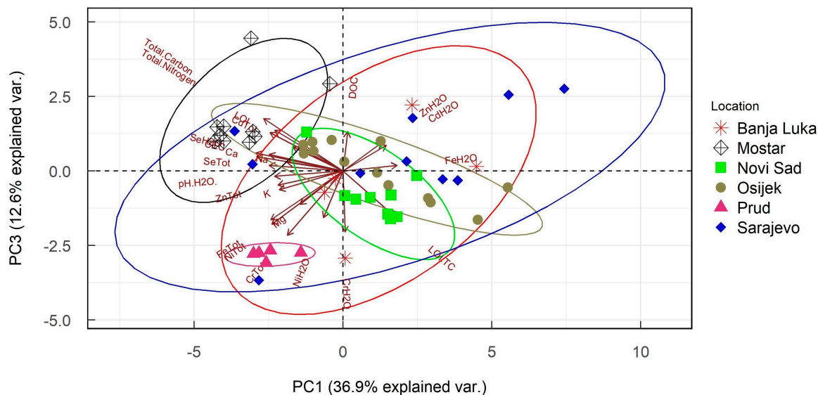
Figure 4. Biplot of principal components 1 and 3 from PCA analysis of variation among six locations with different soil properties. Arrows represent the eigenvectors of each of the 24 selected soil parameters.
