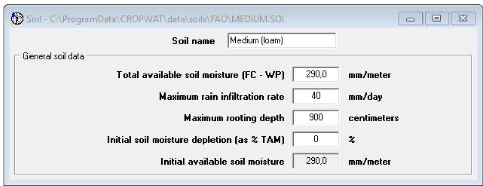
Figure 9. Soil properties
