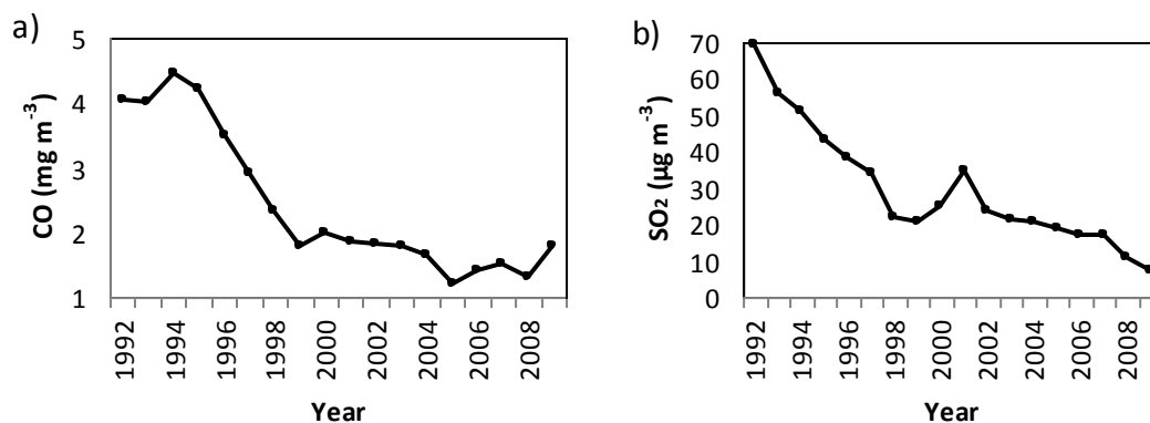
Fig. 1. Annual averages of the (a) CO and (b) SO 2 concentrations in the commercial center of the city (Benizelou monitoring station).
