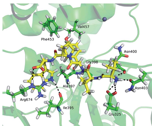
Fig. 6 The tyrosine (carbon atoms are shown in yellow) binding in the yDPP III obtained by MD simulations. Selected amino acid residues interacting with substrate are shown (carbon atoms are shown in green). The intermolecular hydrogen bonds are represented by black dashed lines.
