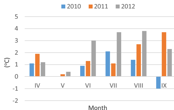
Figure 3. Average air temperature aberrations during 2010 – 2012 period
